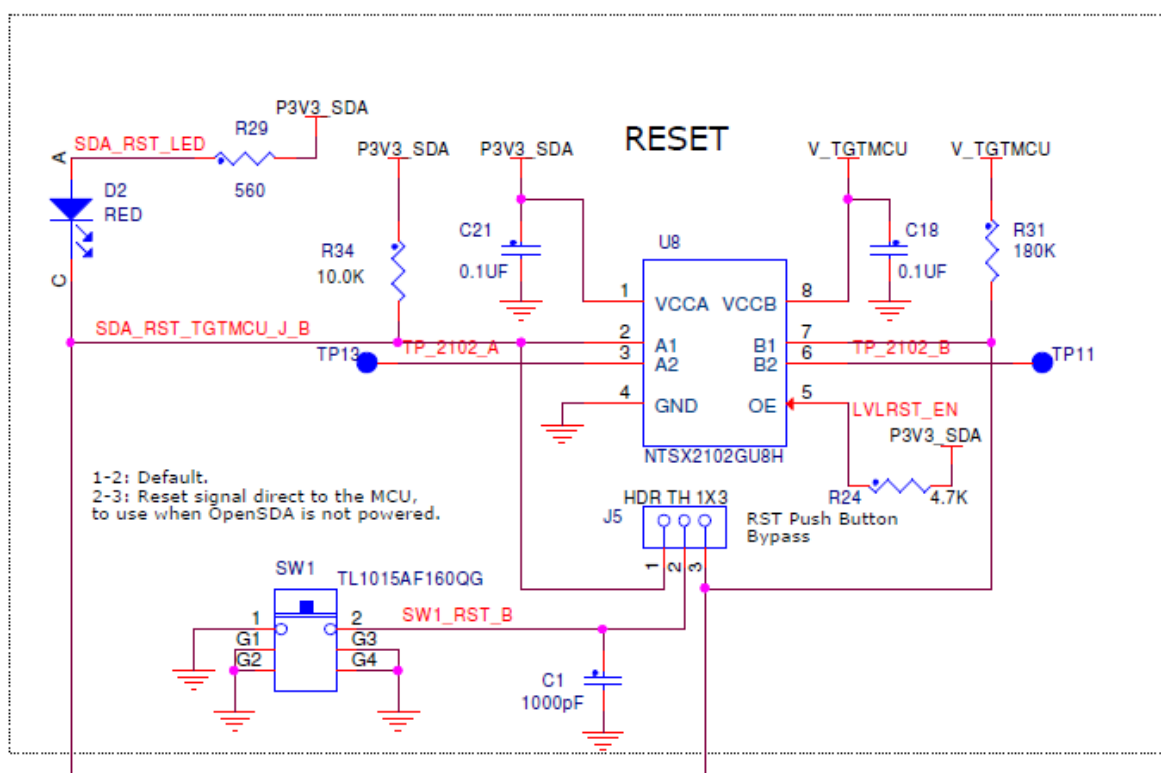
Figure 15. Reset circuit
