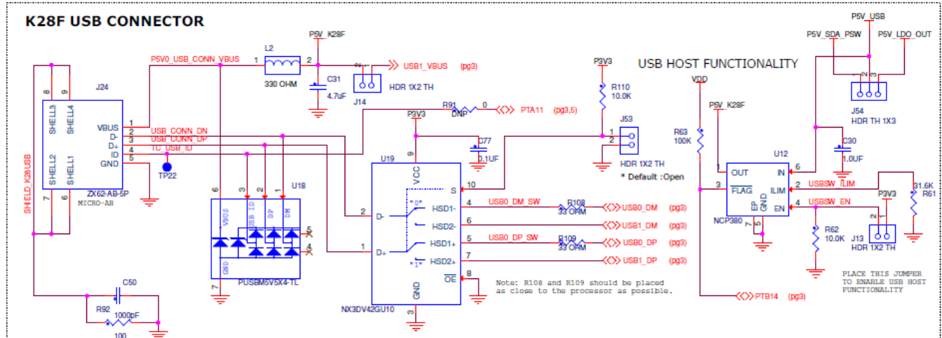
Figure 8. K28F USB port
